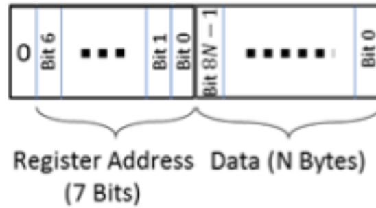
Figure A1-4: LoRaWAN Port 100 Read Response Format
