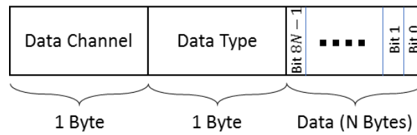
Figure 0-1: The UL Frame Format for Sensor Data Report
