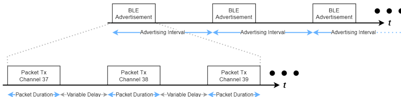
Figure 7-4: The BLE Advertising Scheme
